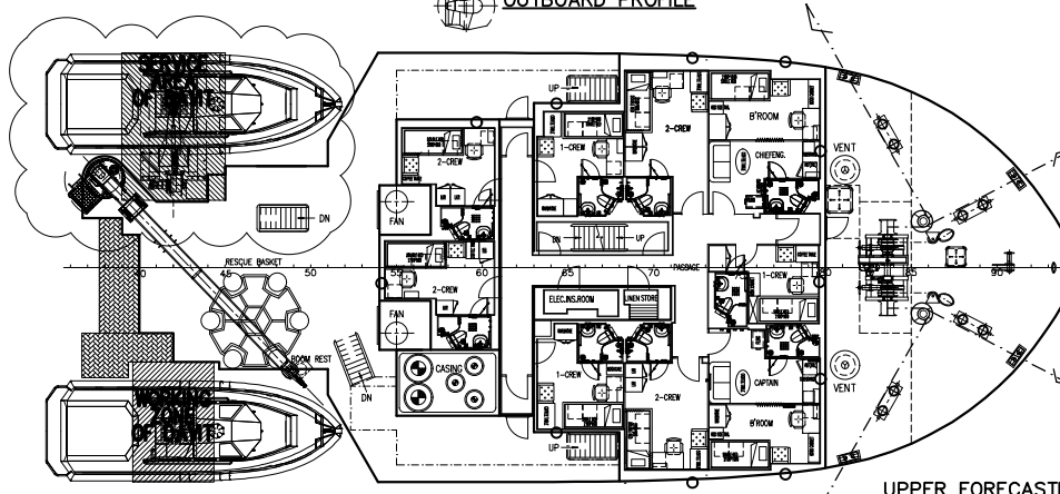
UPPER FORECASTLE DECK 5 x 1-CREW = 5 MEN 4 x 2-CREW = 8 MEN TOTAL = 13 MEN
