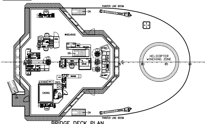
BRIDGE DECK PLAN
