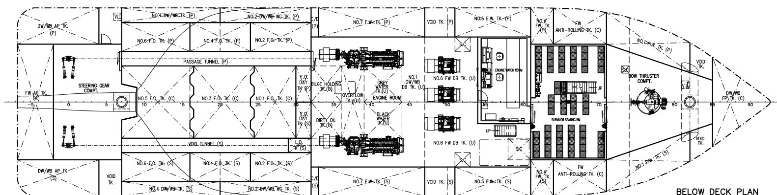
BELOW DECK PLAN
