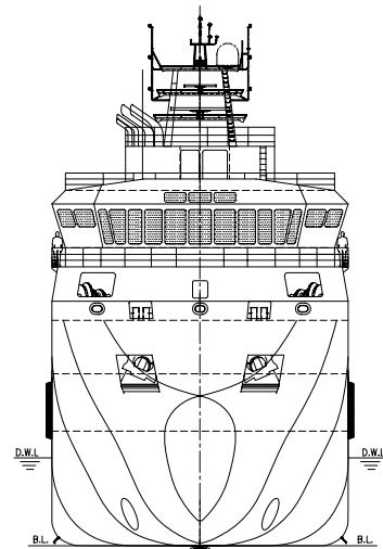
FRONT VIEW (LKG AFT)
