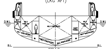
FRONT VIEW (LKG AFT)
