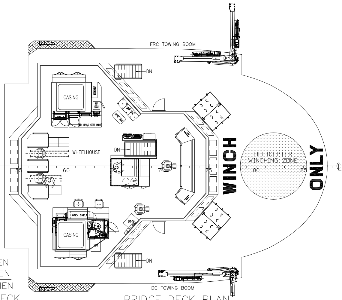
BRIDGE DECK PLAN
