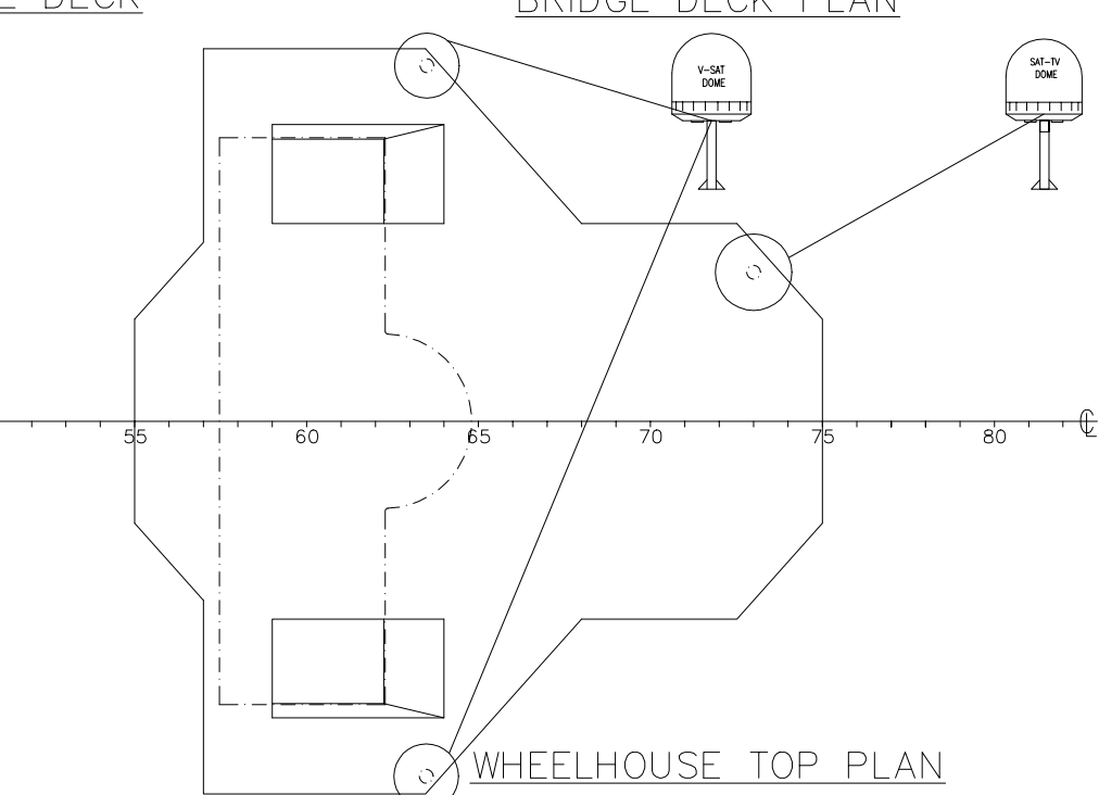
WHEELHOUSE TOP PLAN
