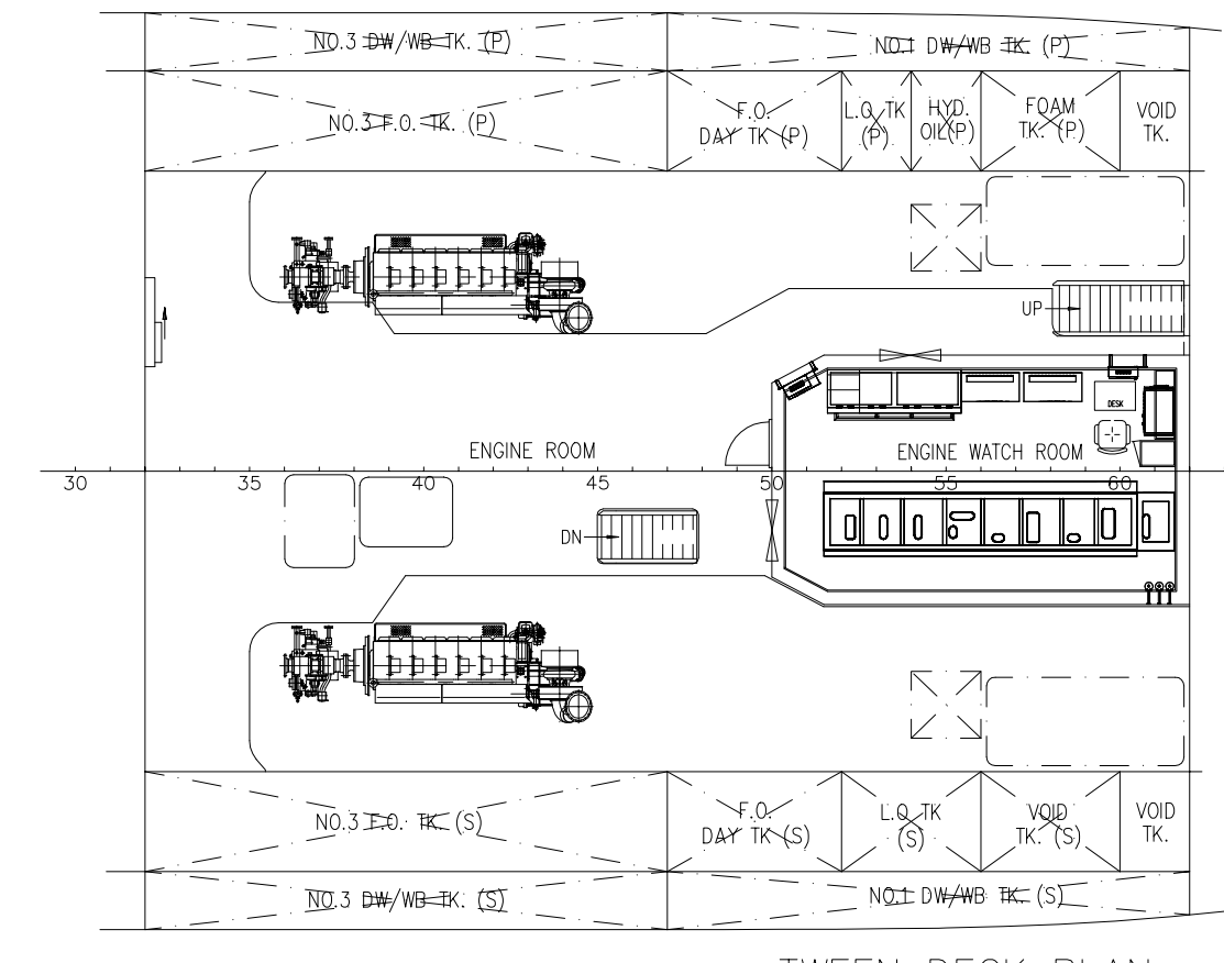
TWEEN DECK PLAN
