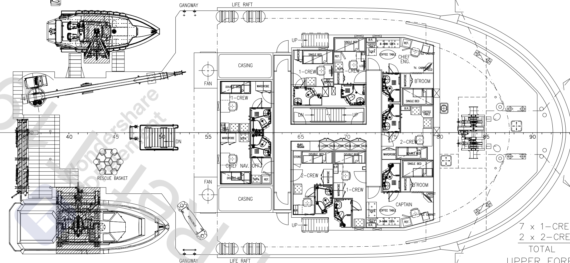
UPPER FORECASTLE DECK
